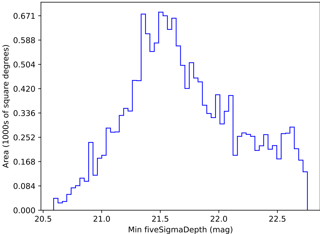
extra_ss_neo3_v3.4_10yrs WFD i band: Min fiveSigmaDepth
