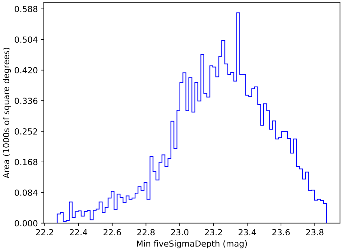
extra_ss_neo3_v3.4_10yrs WFD g band: Min fiveSigmaDepth
