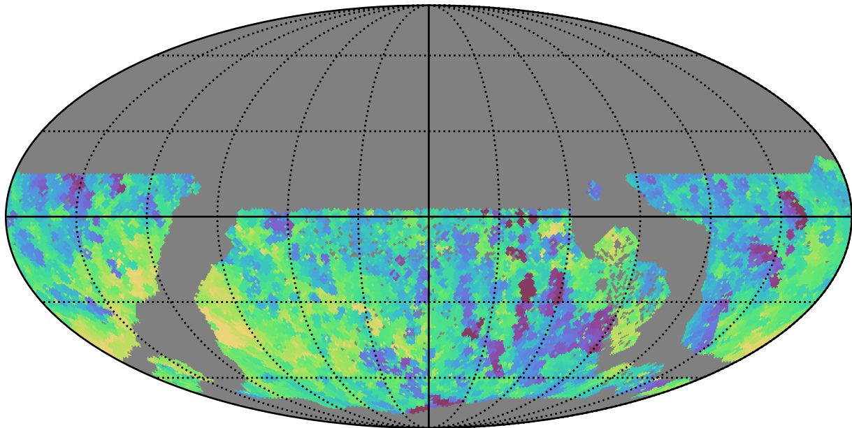
extra_ss_neo3_v3.4_10yrs WFD all bands: Min fiveSigmaDepth
