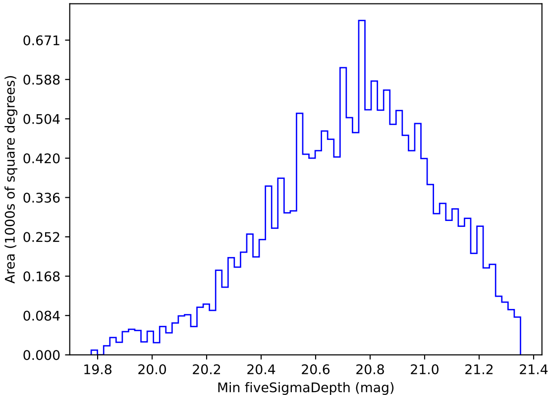
extra_ss_neo3_v3.4_10yrs WFD all bands: Min fiveSigmaDepth
