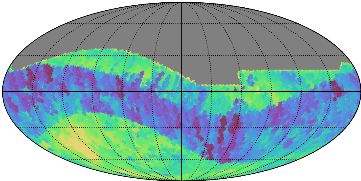
extra_ss_neo3_v3.4_10yrs All sky z band: Min fiveSigmaDepth
