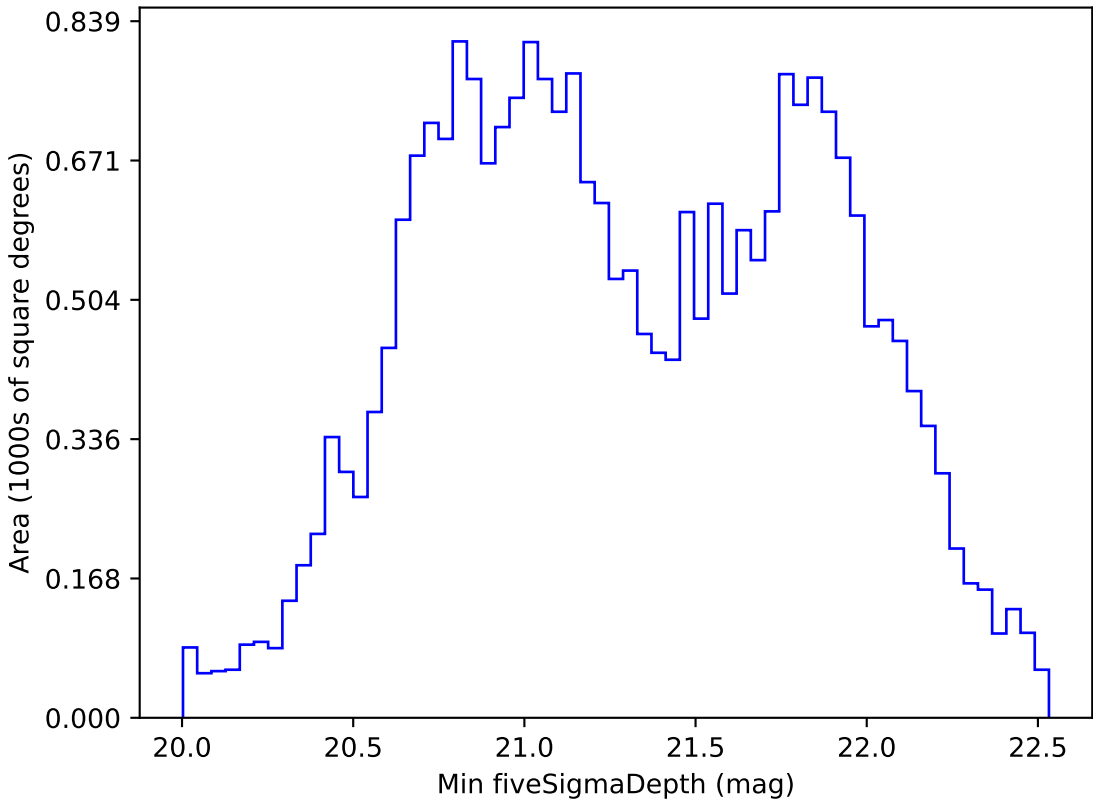
extra_ss_neo3_v3.4_10yrs All sky z band: Min fiveSigmaDepth
