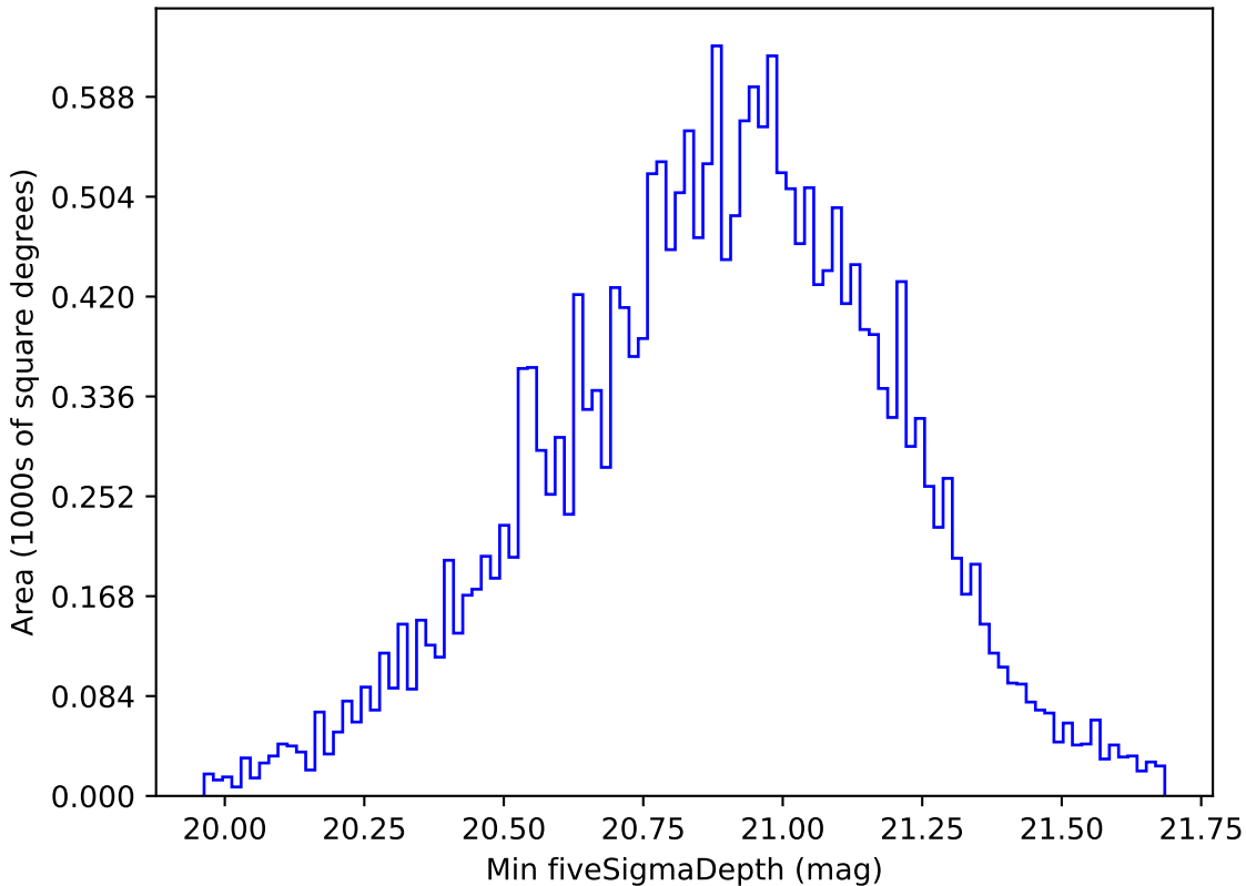
extra_ss_neo3_v3.4_10yrs All sky y band: Min fiveSigmaDepth
