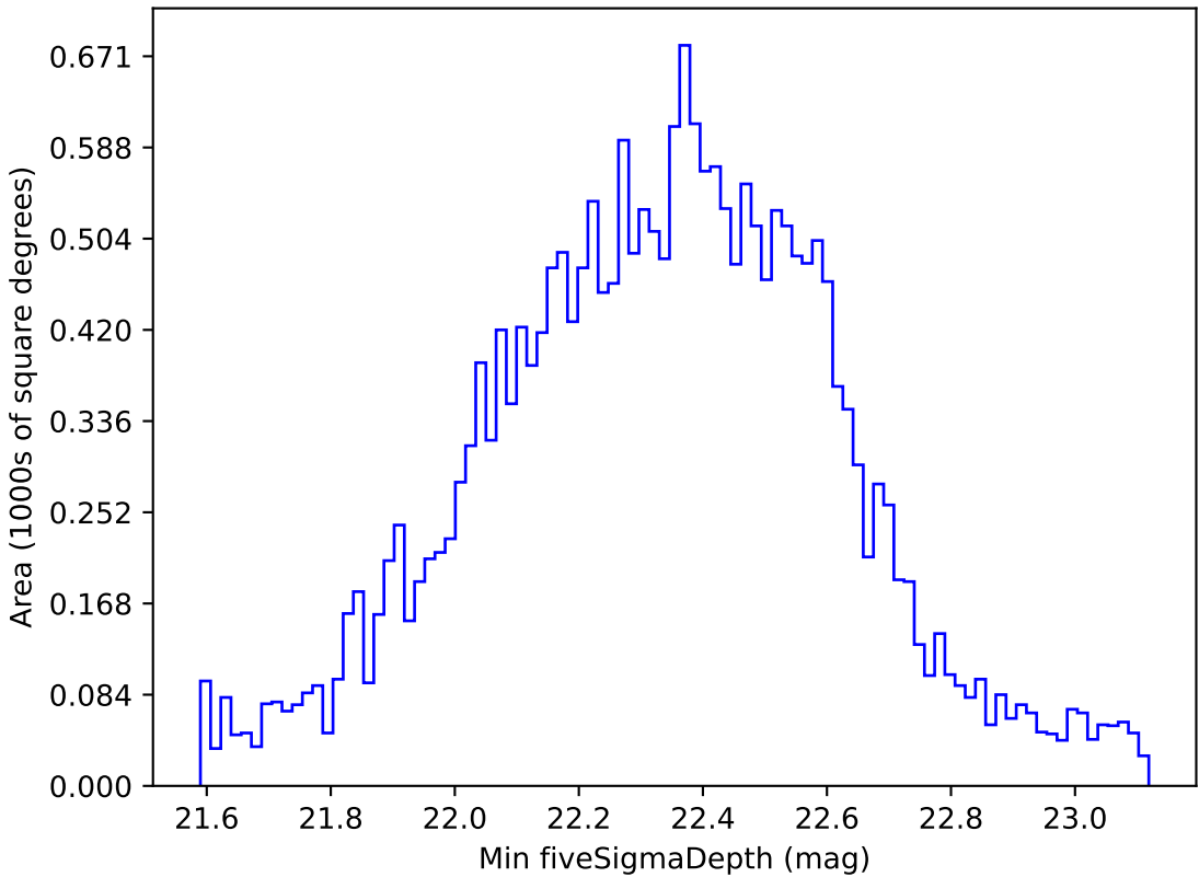
extra_ss_neo3_v3.4_10yrs All sky u band: Min fiveSigmaDepth
