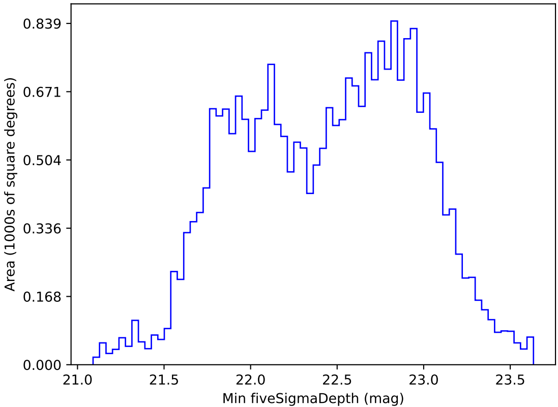
extra_ss_neo3_v3.4_10yrs All sky r band: Min fiveSigmaDepth
