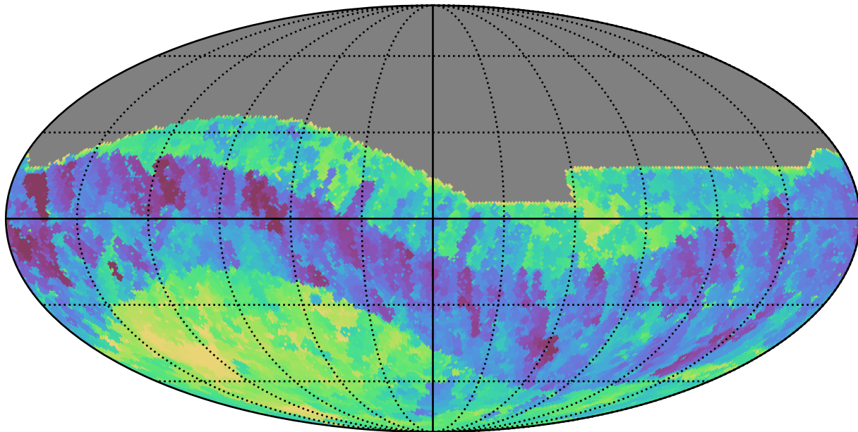
extra_ss_neo3_v3.4_10yrs All sky i band: Min fiveSigmaDepth
