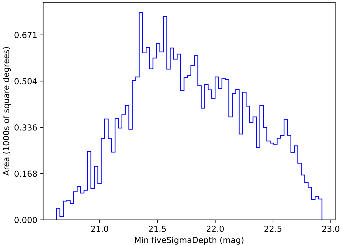
extra_ss_neo3_v3.4_10yrs All sky i band: Min fiveSigmaDepth
