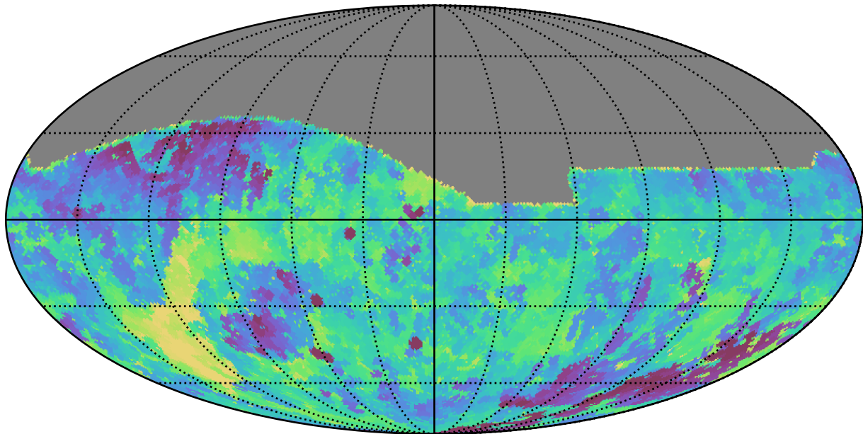
extra_ss_neo3_v3.4_10yrs All sky g band: Min fiveSigmaDepth
