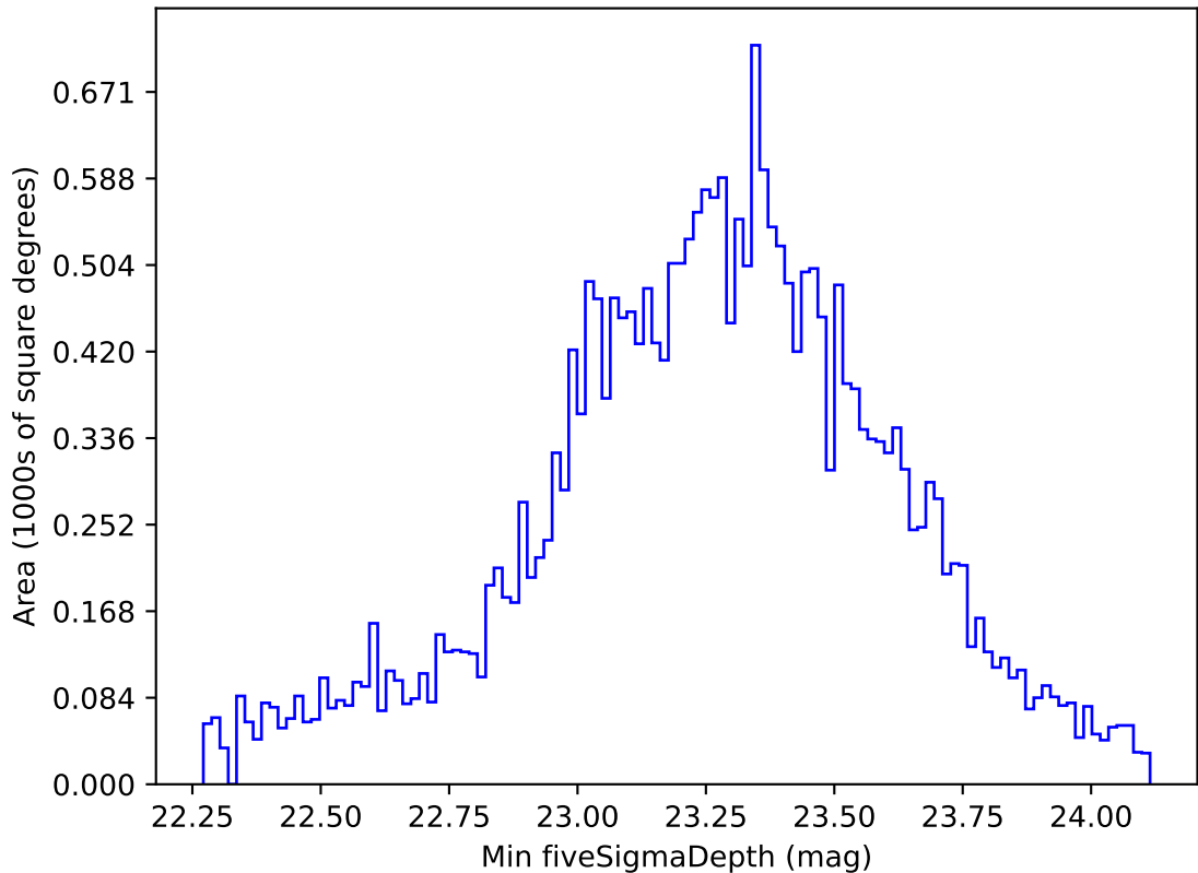
extra_ss_neo3_v3.4_10yrs All sky g band: Min fiveSigmaDepth
