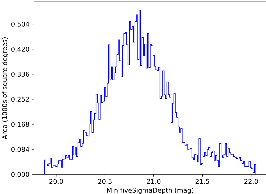
extra_ss_neo3_v3.4_10yrs All sky all bands: Min fiveSigmaDepth
