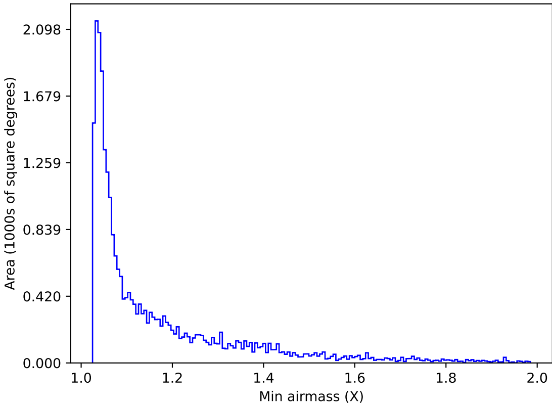
extra_ss_neo3_v3.4_10yrs Yr 1 z band: Min airmass
