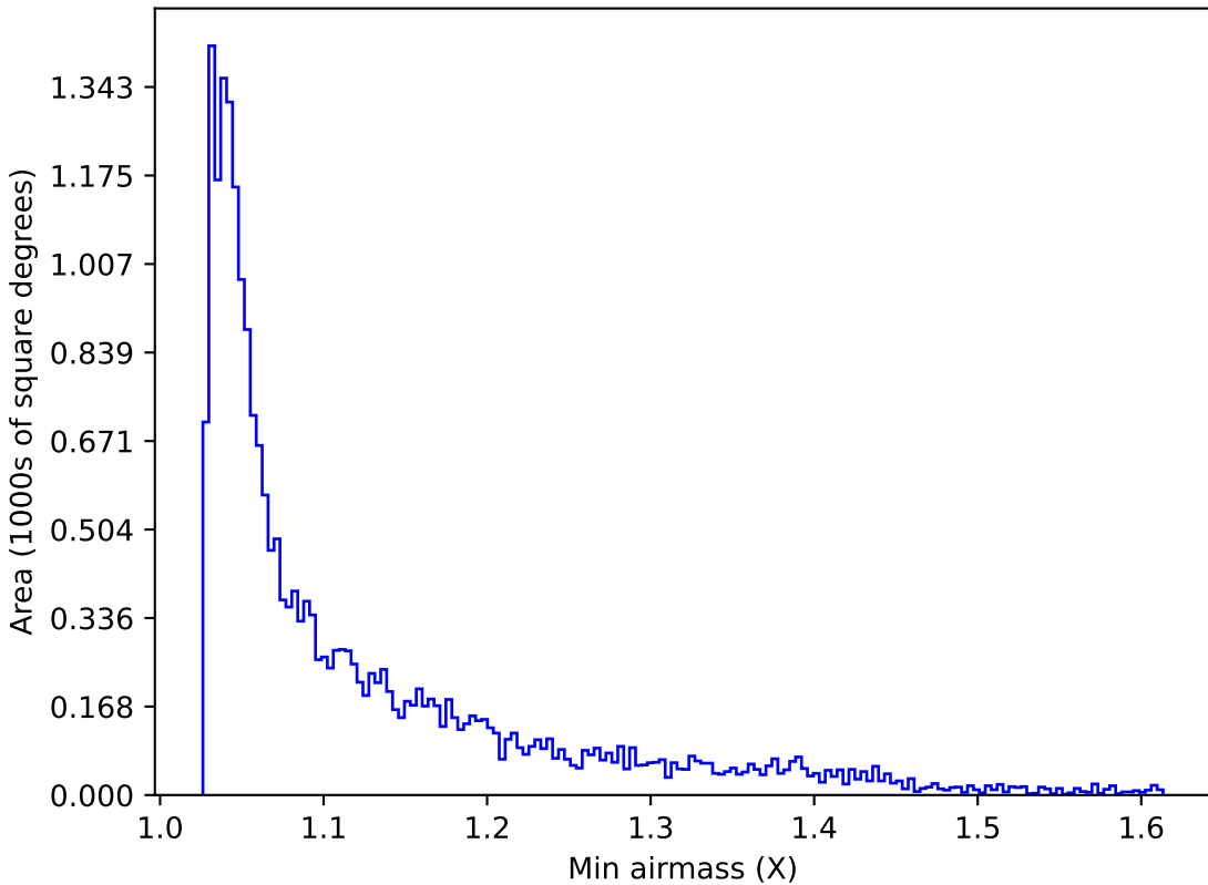
extra_ss_neo3_v3.4_10yrs Yr 1 y band: Min airmass
