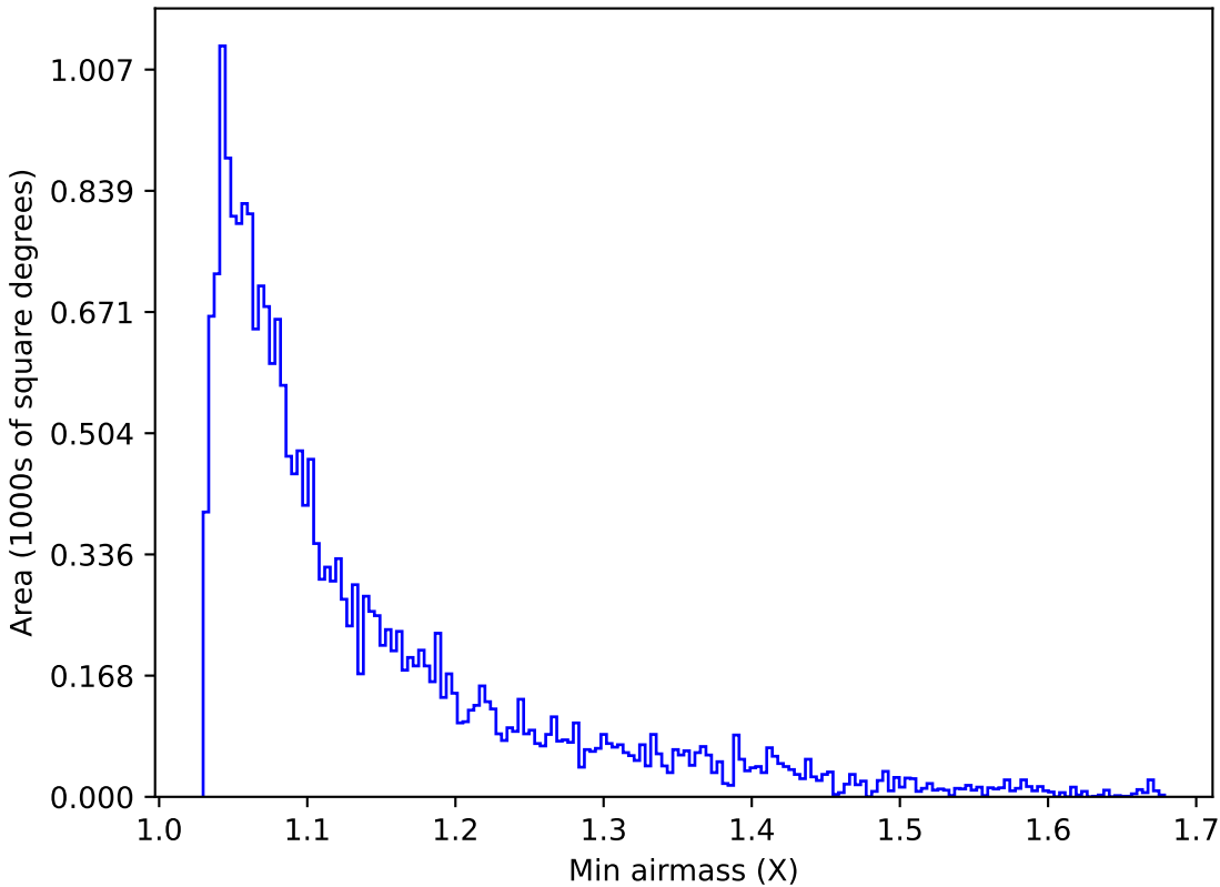
extra_ss_neo3_v3.4_10yrs Yr 1 u band: Min airmass
