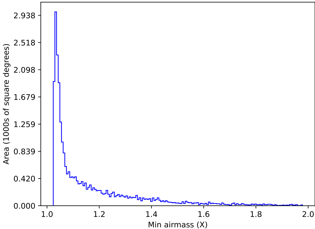
extra_ss_neo3_v3.4_10yrs Yr 1 r band: Min airmass
