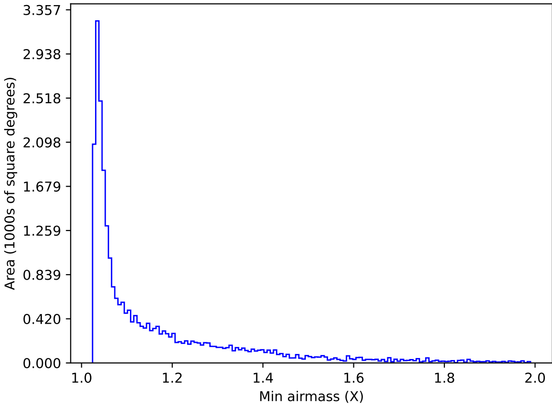
extra_ss_neo3_v3.4_10yrs Yr 1 i band: Min airmass
