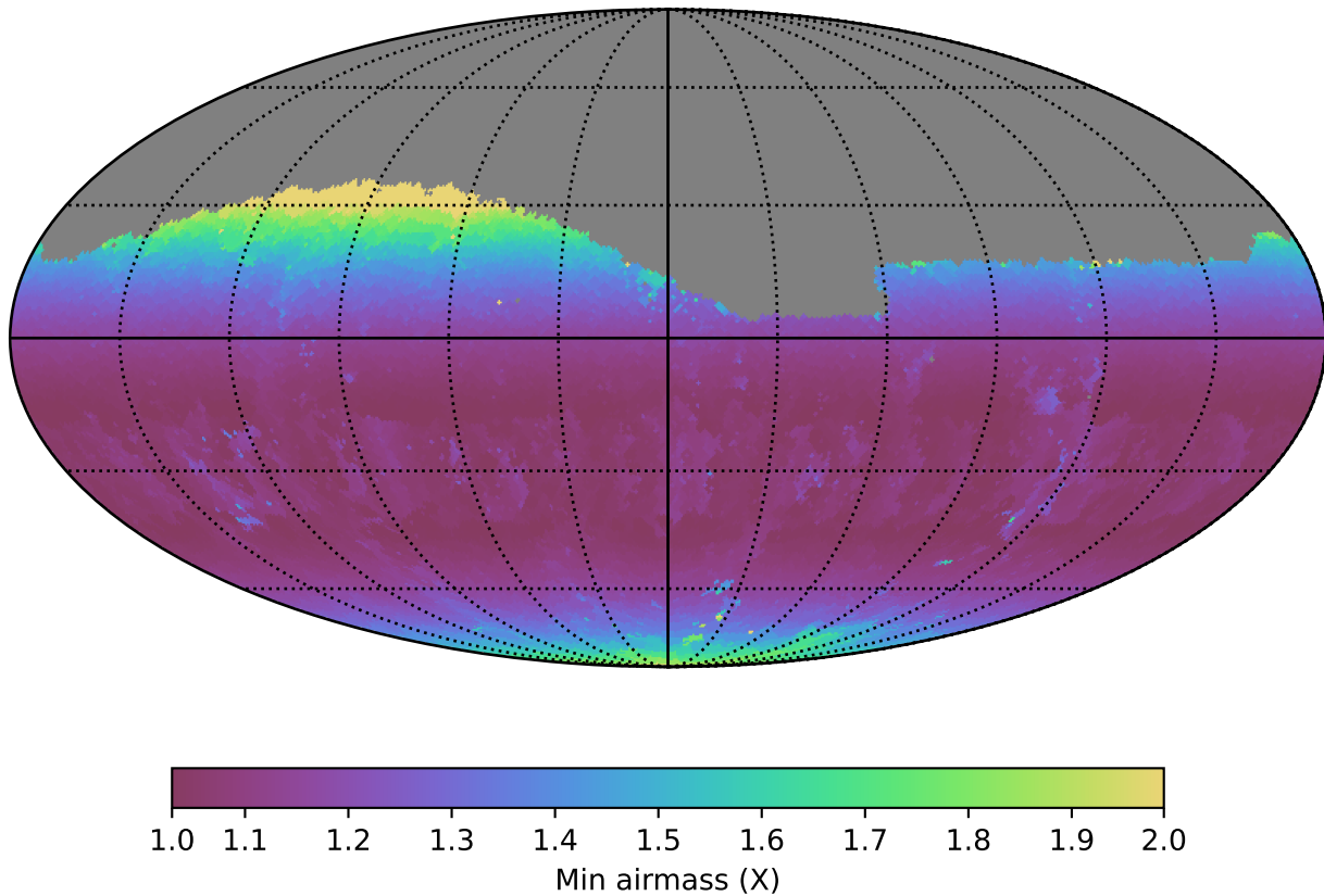
extra_ss_neo3_v3.4_10yrs Yr 1 g band: Min airmass
