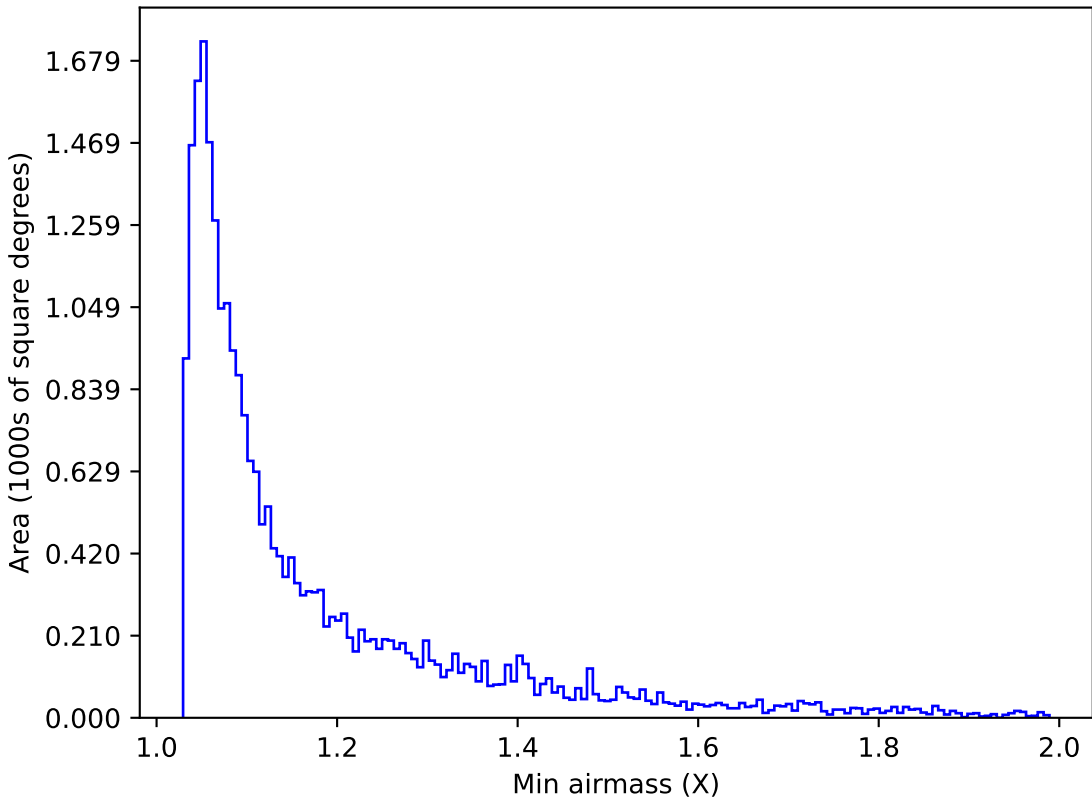
extra_ss_neo3_v3.4_10yrs Yr 1 g band: Min airmass
