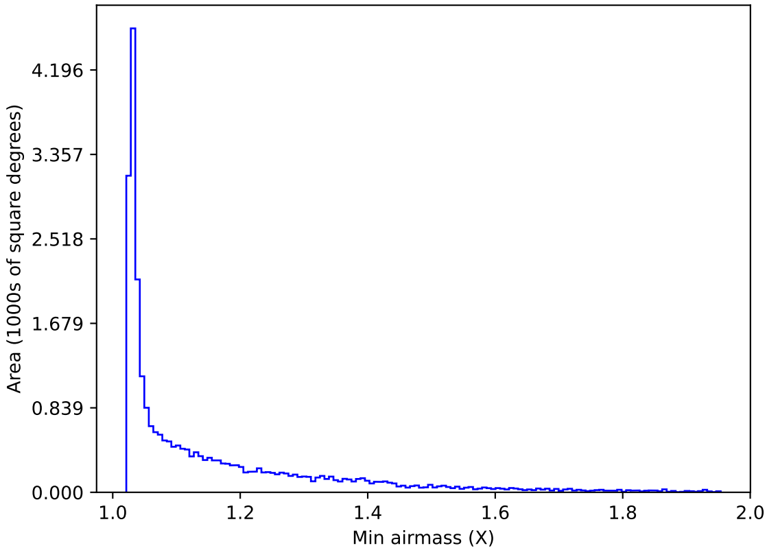
extra_ss_neo3_v3.4_10yrs Yr 1 all bands: Min airmass
