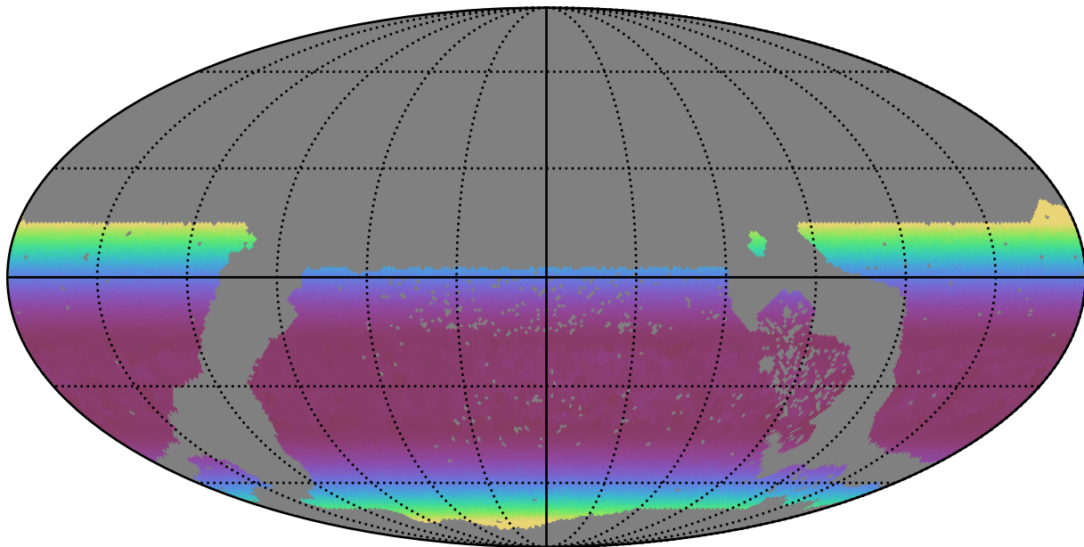
extra_ss_neo3_v3.4_10yrs WFD z band: Min airmass
