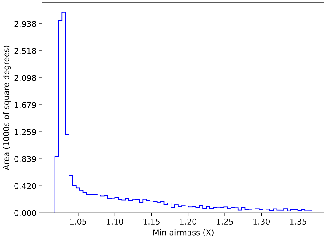
extra_ss_neo3_v3.4_10yrs WFD z band: Min airmass
