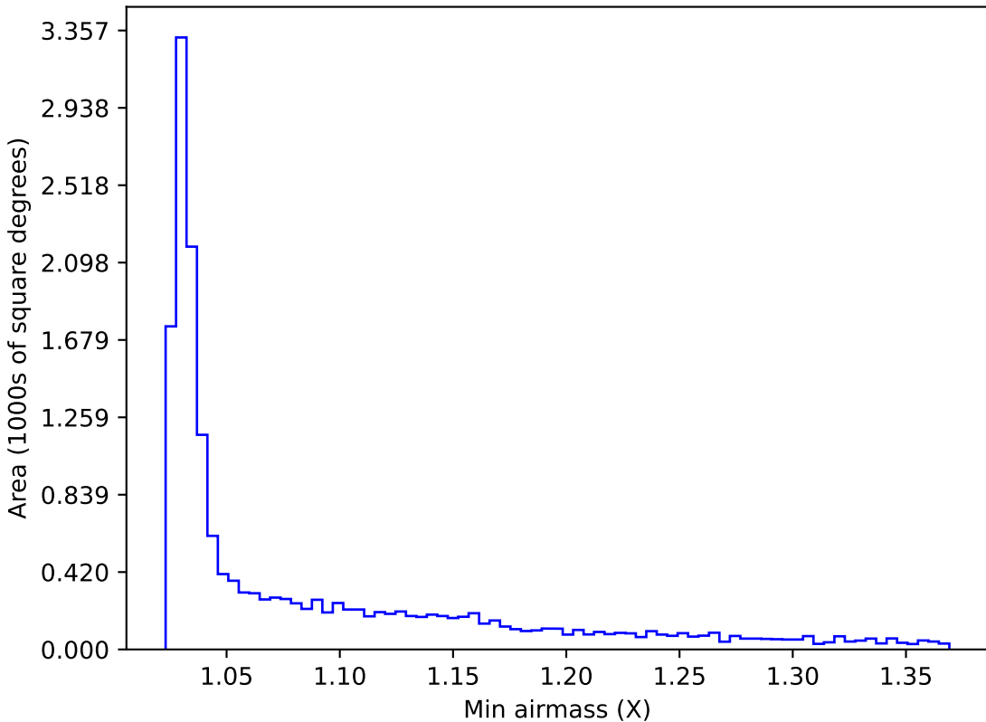
extra_ss_neo3_v3.4_10yrs WFD y band: Min airmass
