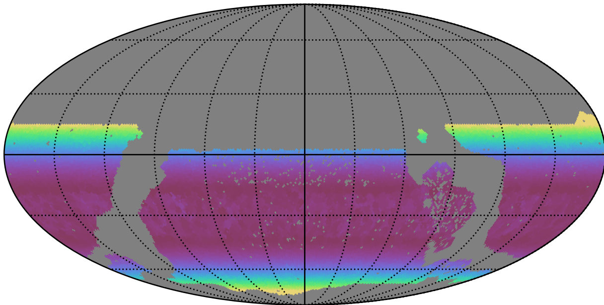
extra_ss_neo3_v3.4_10yrs WFD u band: Min airmass
