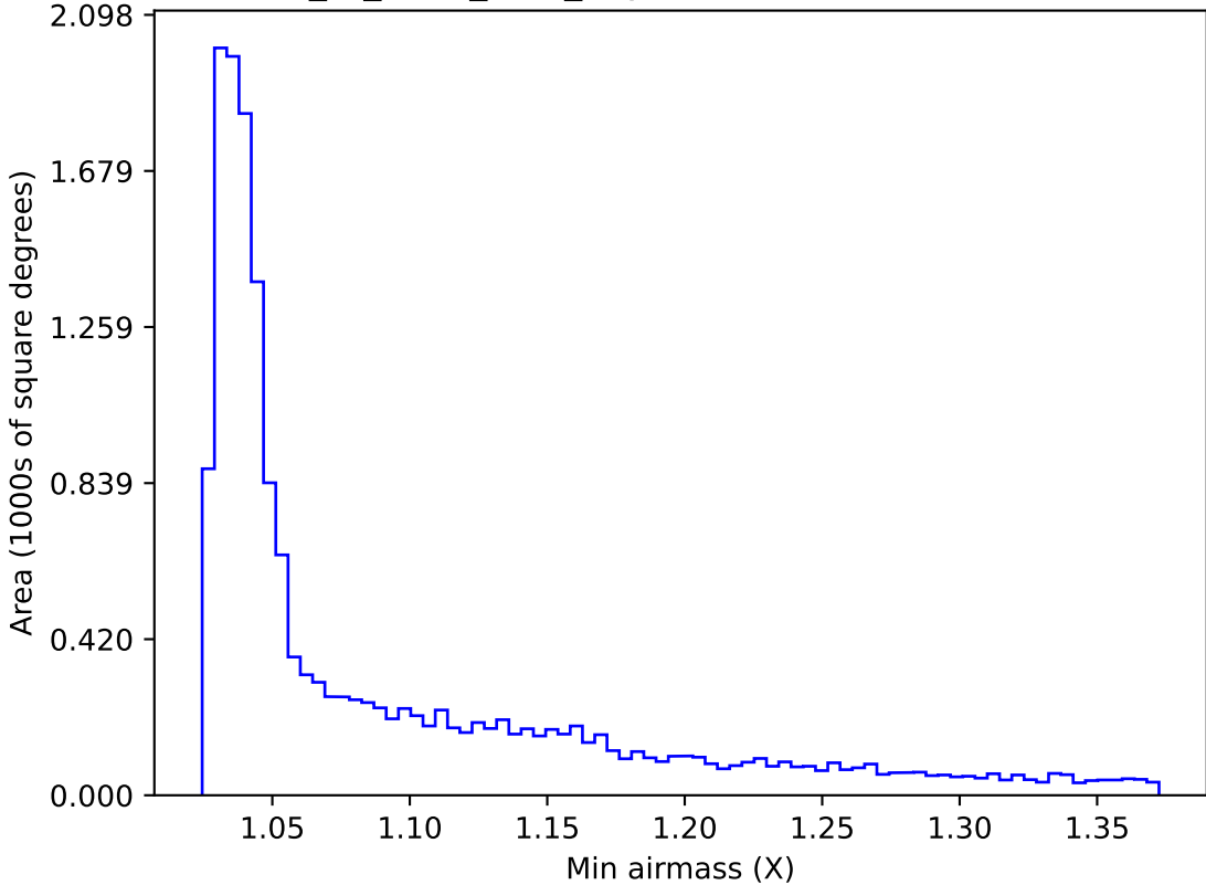
extra_ss_neo3_v3.4_10yrs WFD u band: Min airmass
