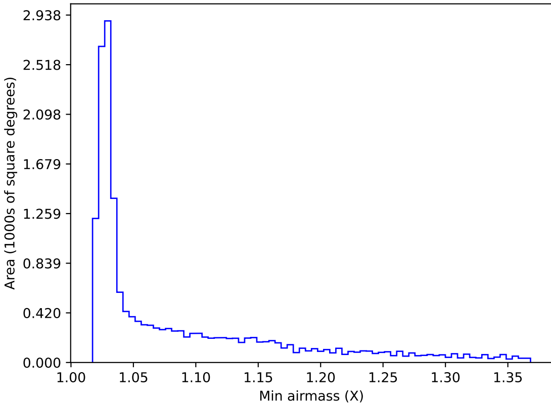
extra_ss_neo3_v3.4_10yrs WFD r band: Min airmass
