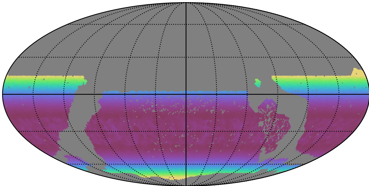
extra_ss_neo3_v3.4_10yrs WFD g band: Min airmass
