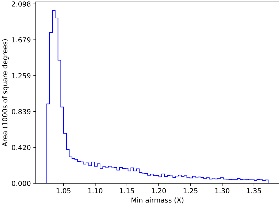
extra_ss_neo3_v3.4_10yrs WFD g band: Min airmass
