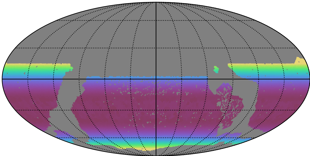
extra_ss_neo3_v3.4_10yrs WFD all bands: Min airmass
