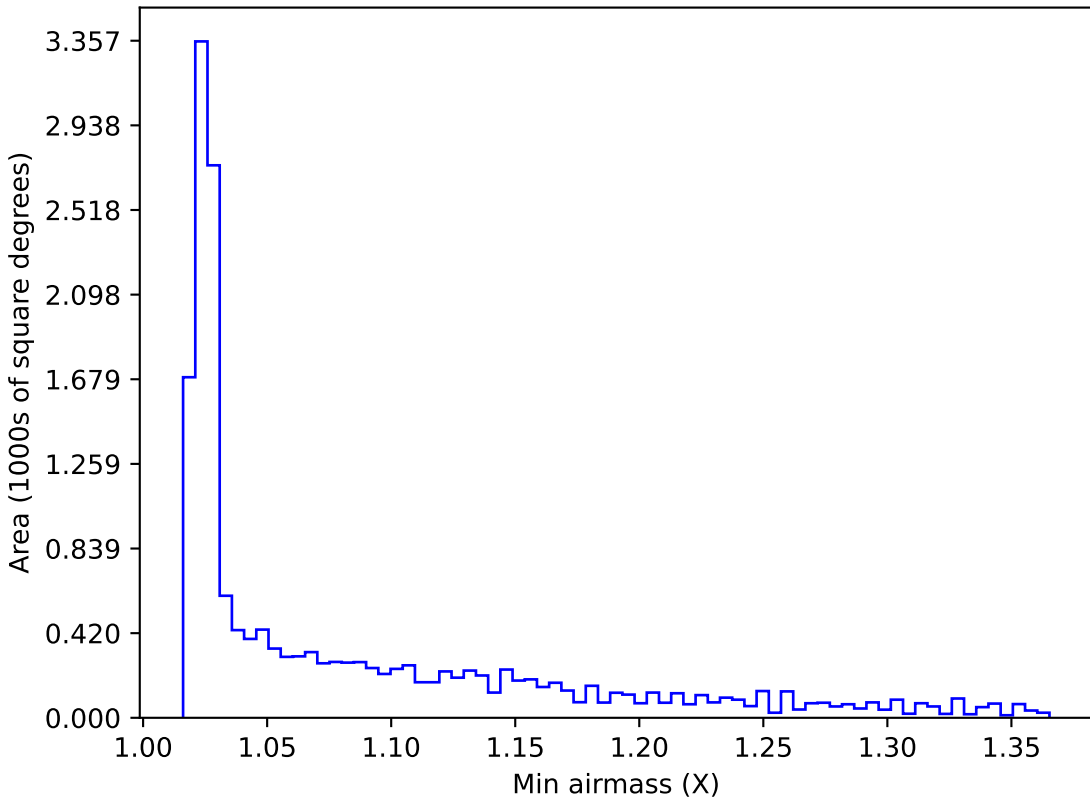
extra_ss_neo3_v3.4_10yrs WFD all bands: Min airmass
