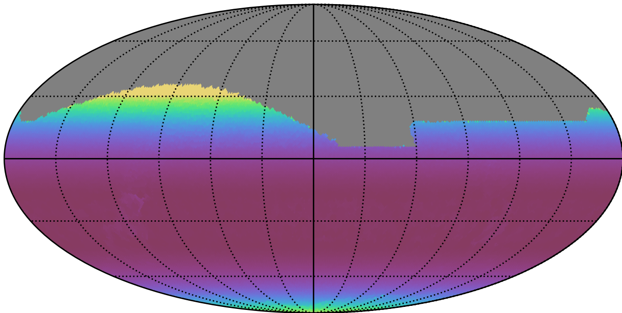
extra_ss_neo3_v3.4_10yrs All sky z band: Min airmass
