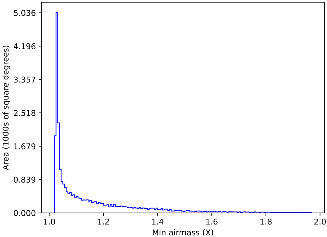
extra_ss_neo3_v3.4_10yrs All sky z band: Min airmass
