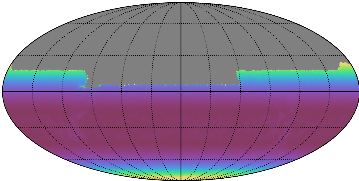
extra_ss_neo3_v3.4_10yrs All sky y band: Min airmass
