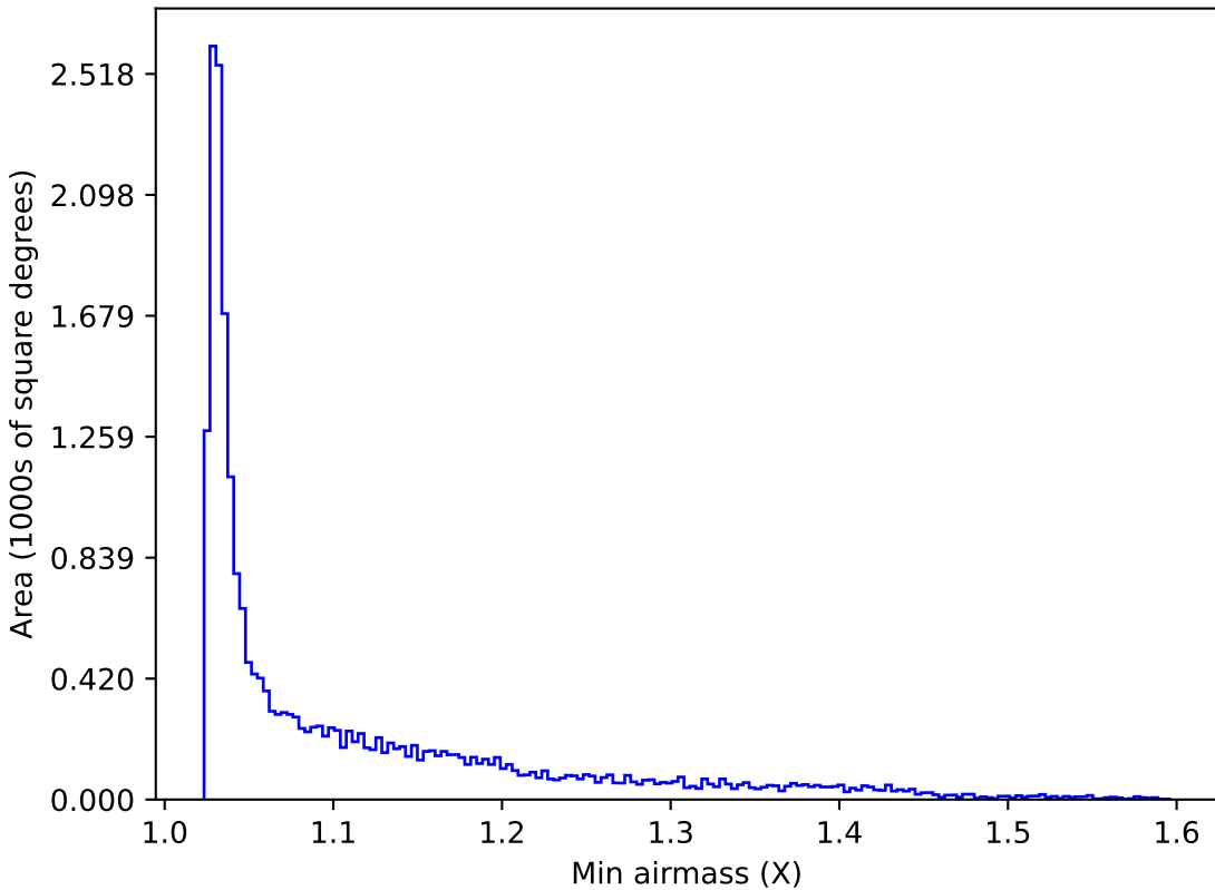
extra_ss_neo3_v3.4_10yrs All sky y band: Min airmass
