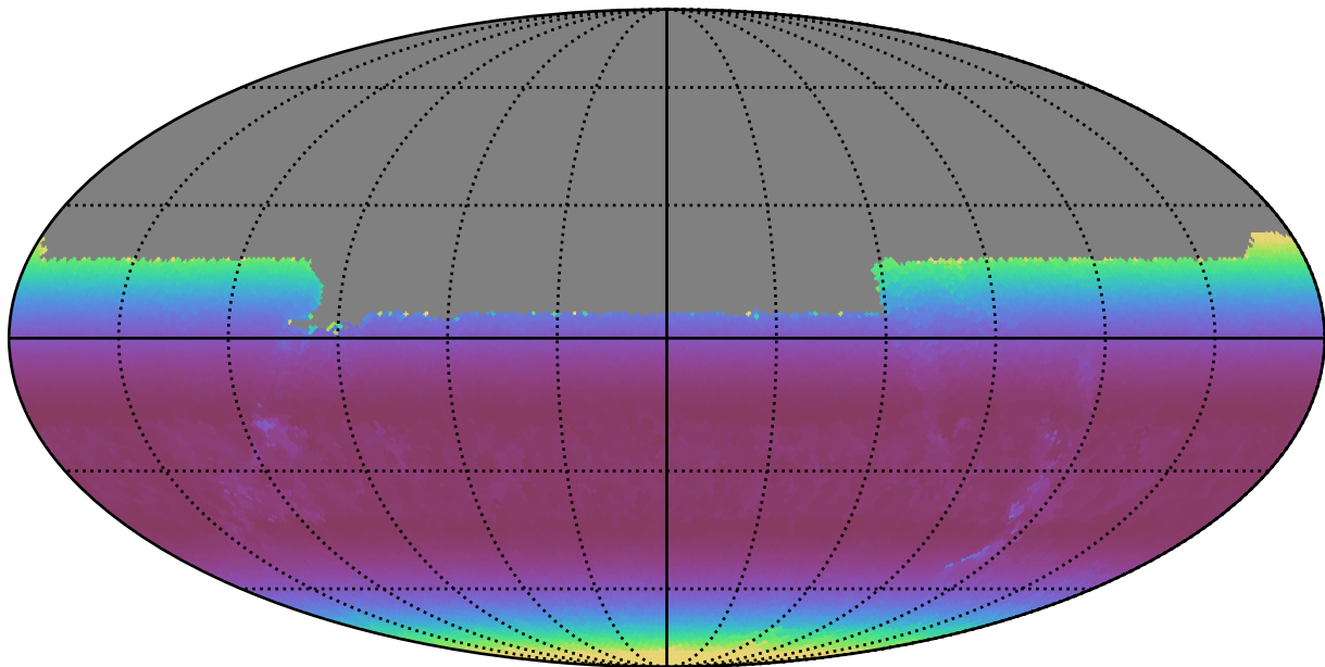
extra_ss_neo3_v3.4_10yrs All sky u band: Min airmass
