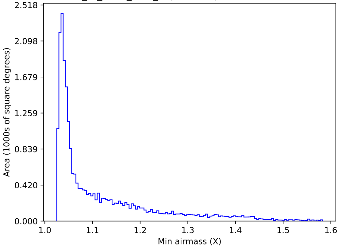
extra_ss_neo3_v3.4_10yrs All sky u band: Min airmass
