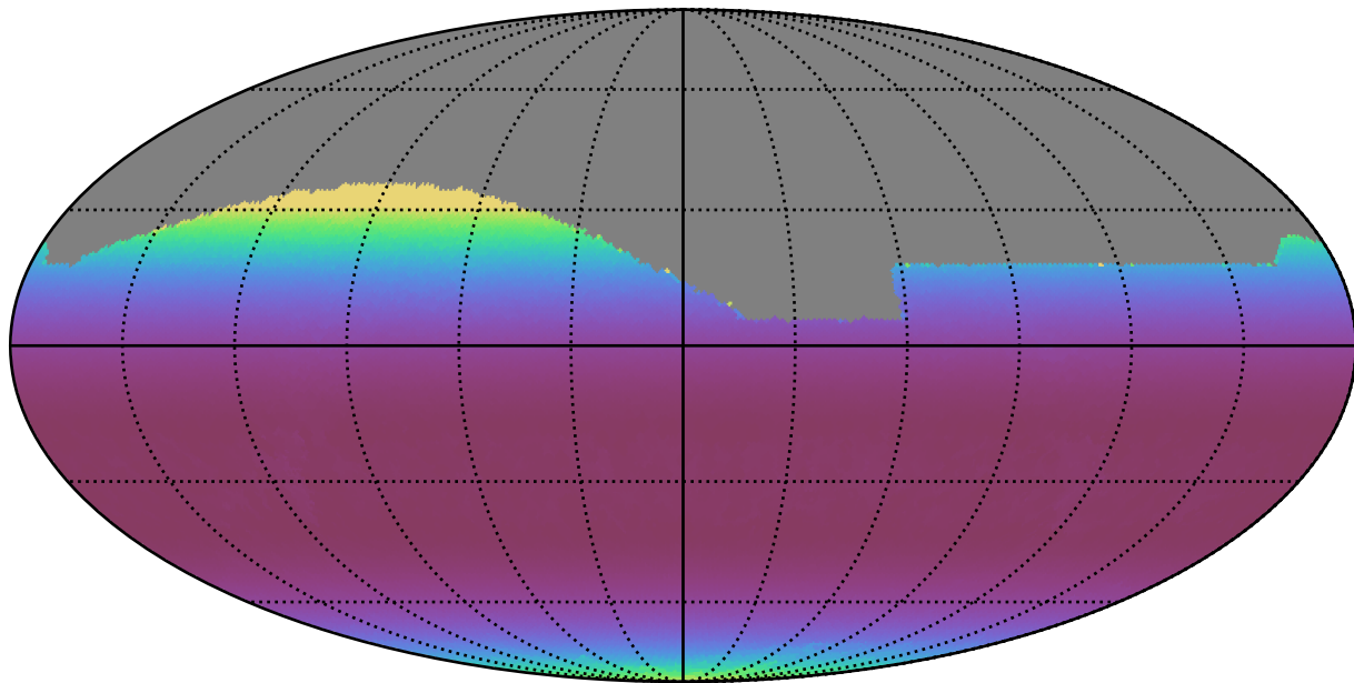
extra_ss_neo3_v3.4_10yrs All sky r band: Min airmass
