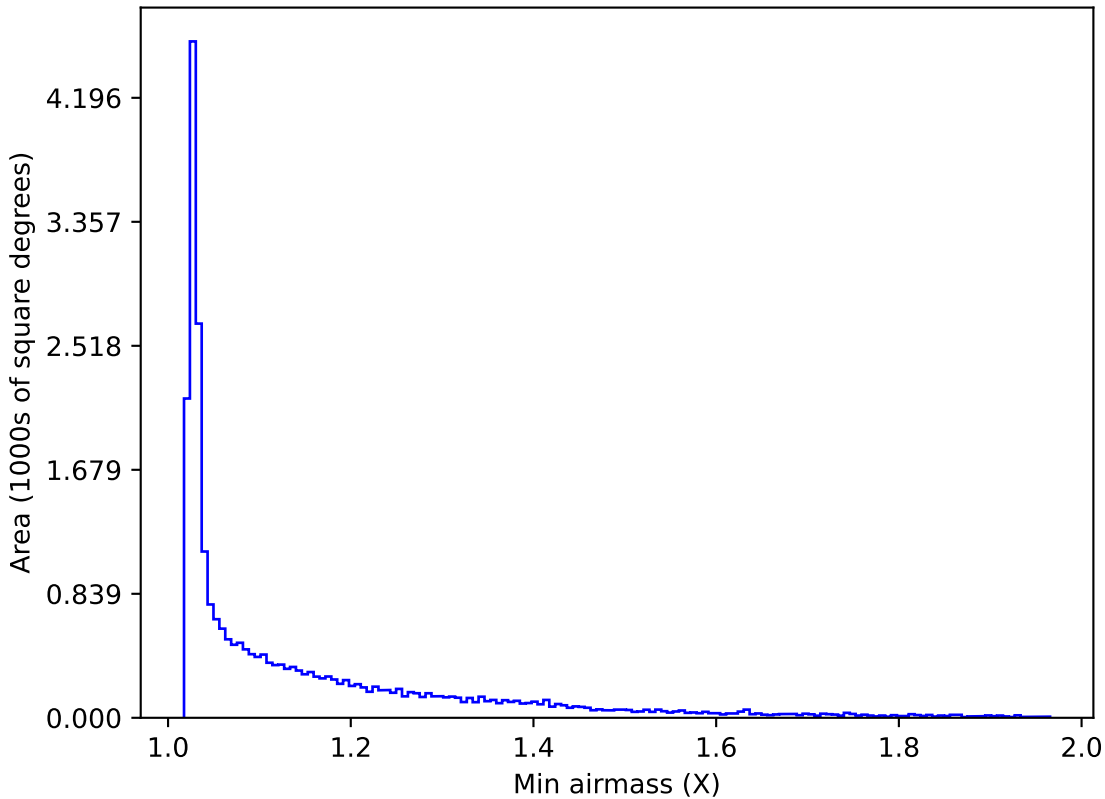
extra_ss_neo3_v3.4_10yrs All sky r band: Min airmass
