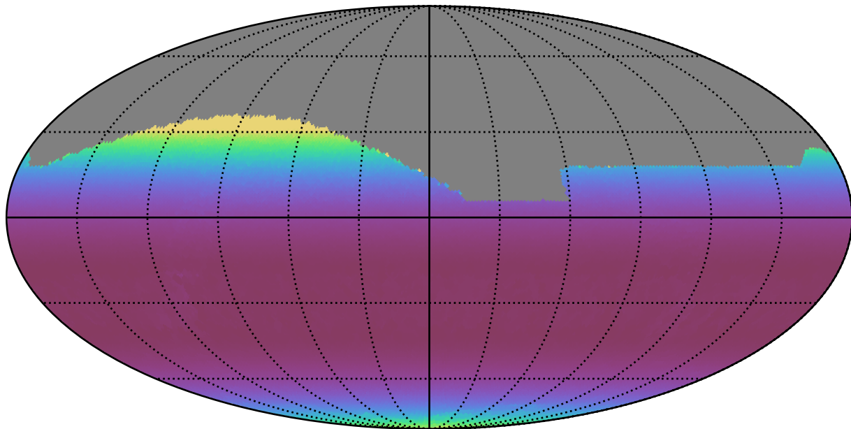
extra_ss_neo3_v3.4_10yrs All sky i band: Min airmass
