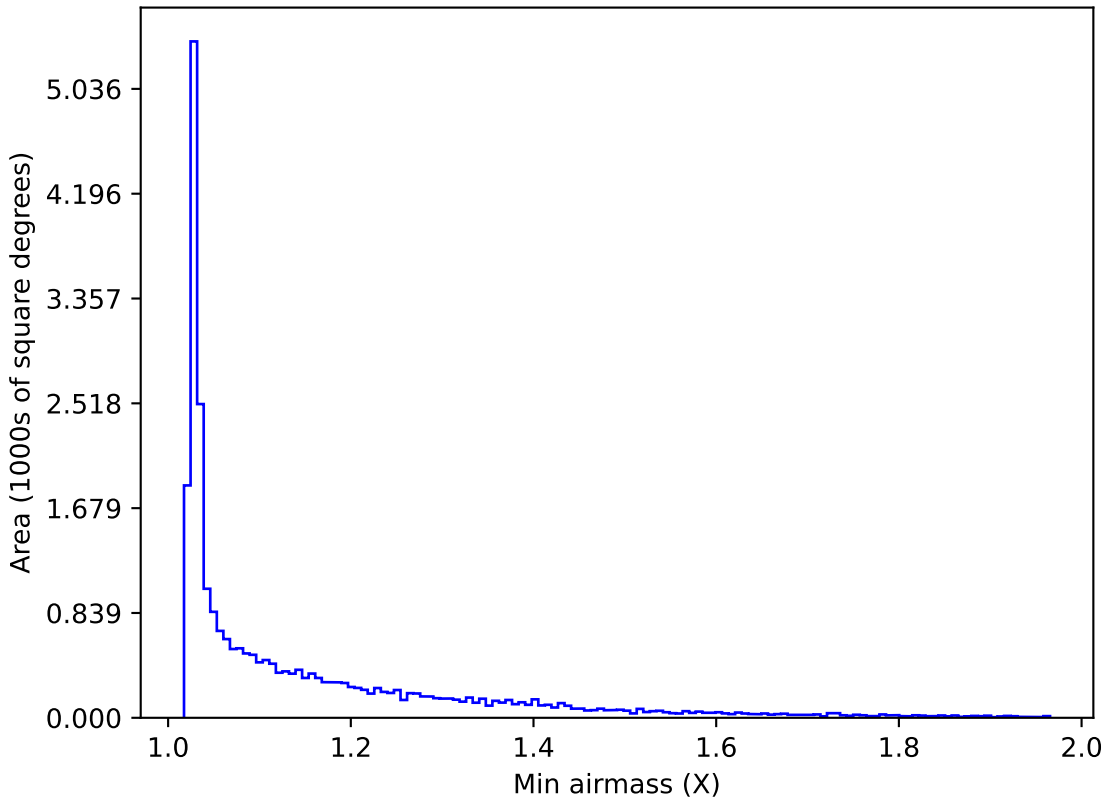
extra_ss_neo3_v3.4_10yrs All sky i band: Min airmass
