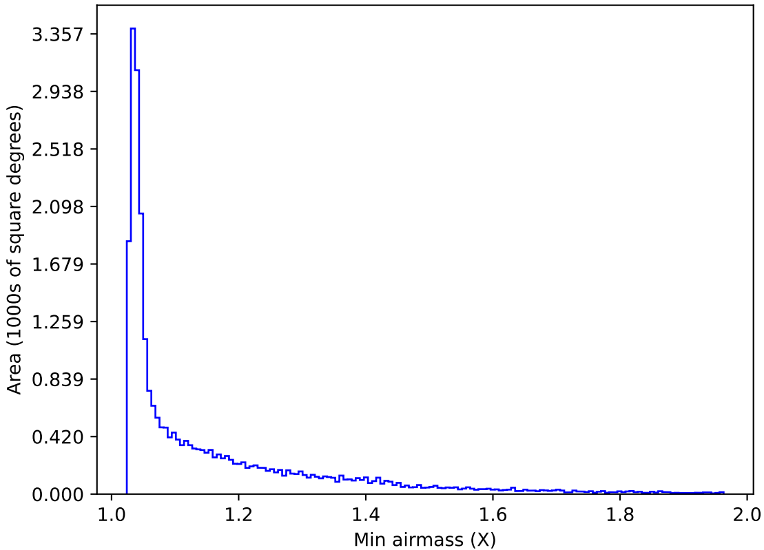
extra_ss_neo3_v3.4_10yrs All sky g band: Min airmass
