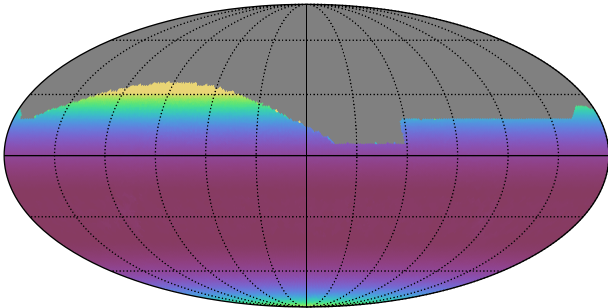
extra_ss_neo3_v3.4_10yrs All sky all bands: Min airmass
