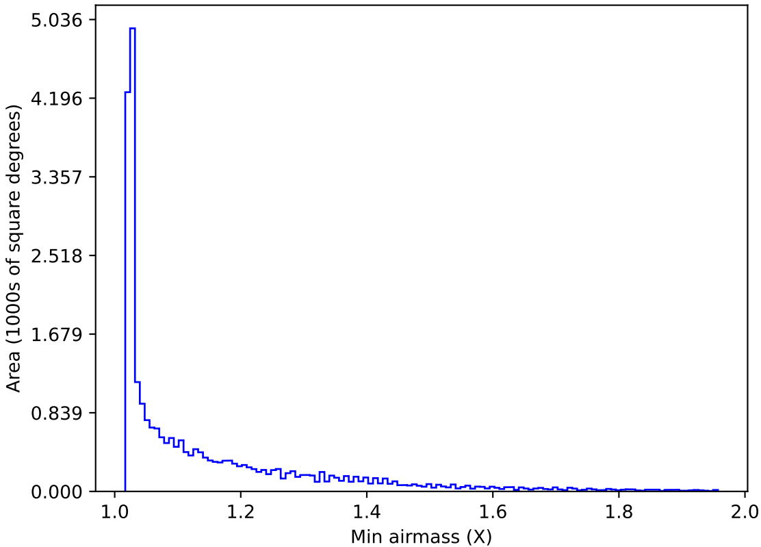
extra_ss_neo3_v3.4_10yrs All sky all bands: Min airmass
