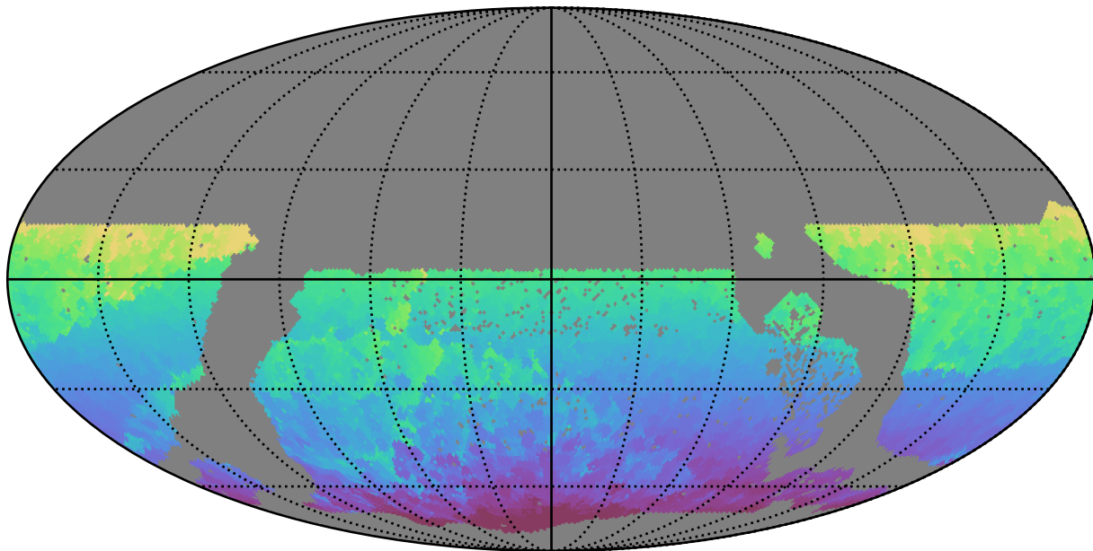
extra_ss_neo3_v3.4_10yrs WFD all bands: Min HA
