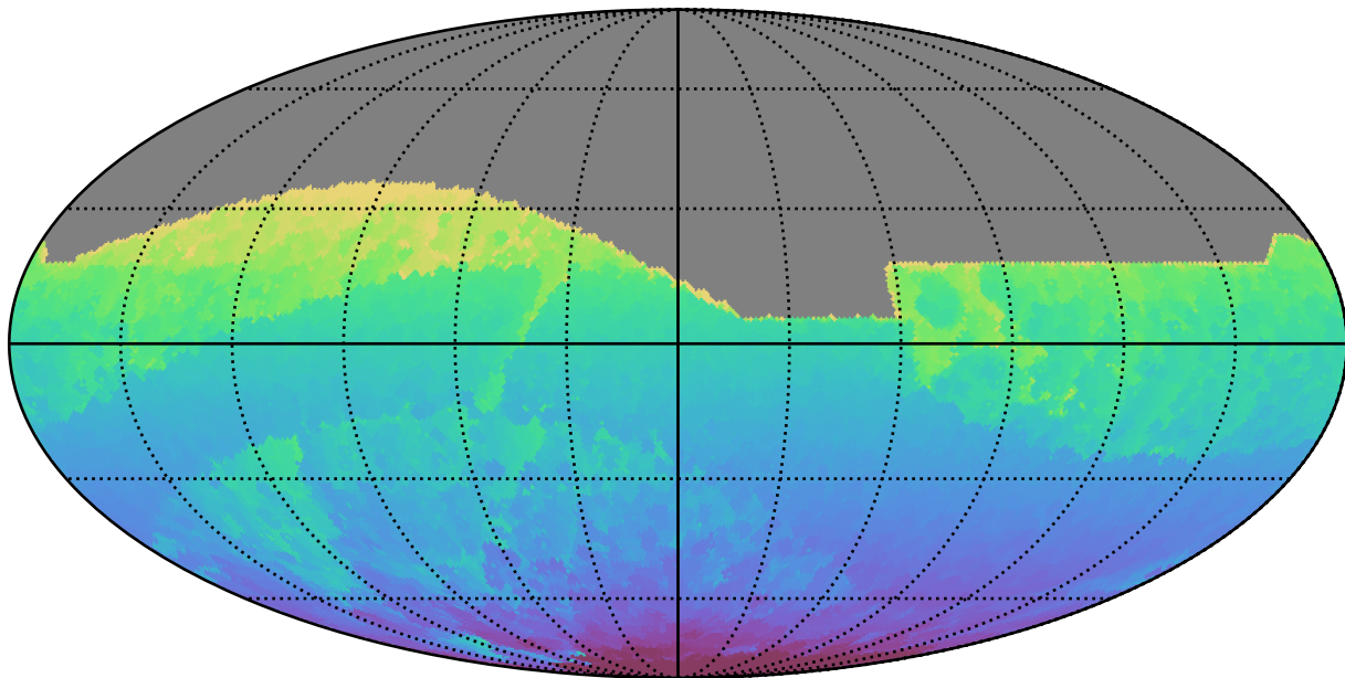
extra_ss_neo3_v3.4_10yrs All sky all bands: Min HA
