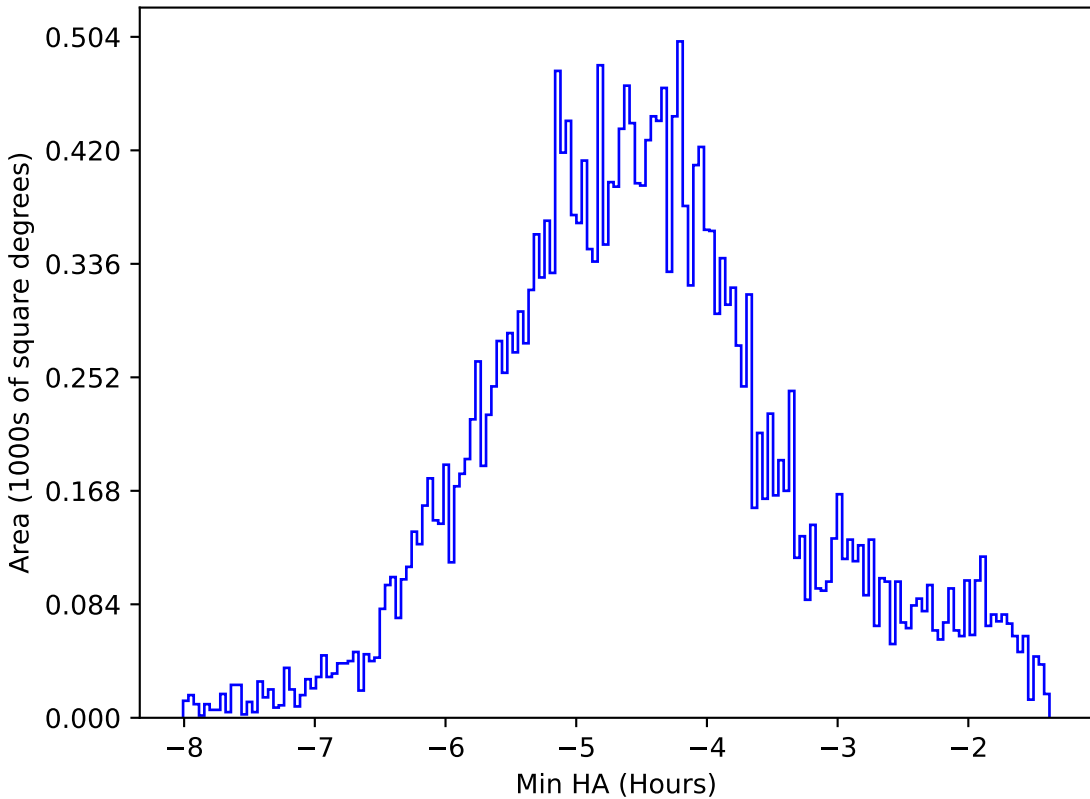
extra_ss_neo3_v3.4_10yrs All sky all bands: Min HA
