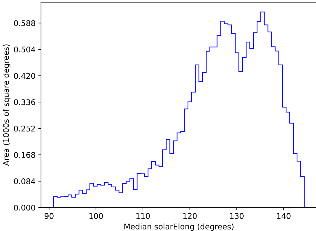
extra_ss_neo3_v3.4_10yrs WFD z band: Median solarElong
