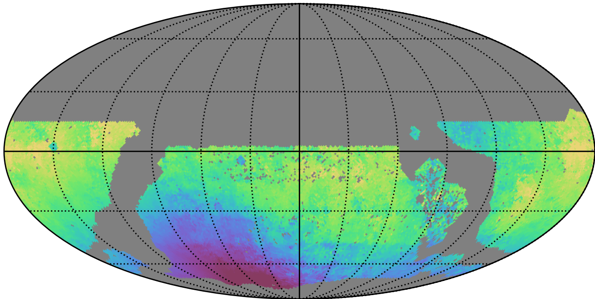
extra_ss_neo3_v3.4_10yrs WFD u band: Median solarElong
